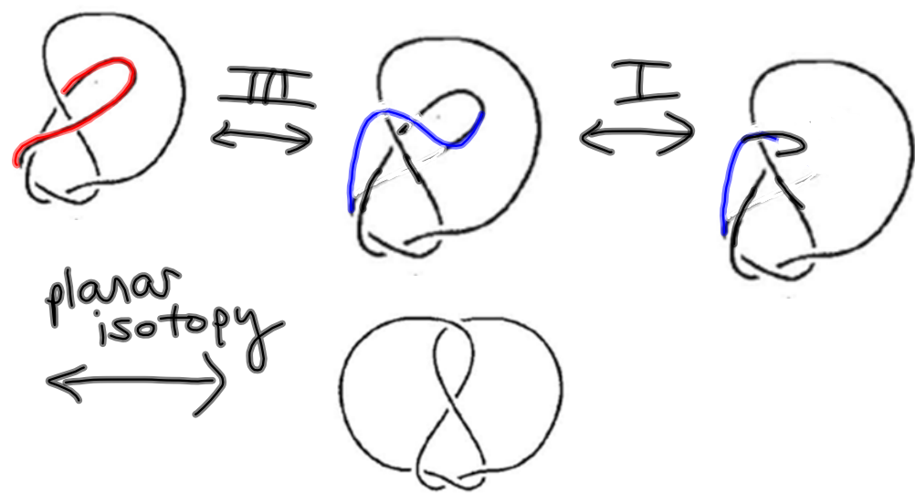
Figure 1.25 Two projections of the same knot.
