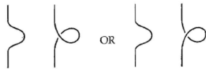
Figure 1.22 Type I Reidemeister move.
