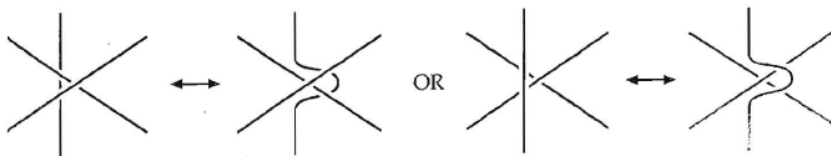
Figure 1.24 Type III Reidemeister move.
