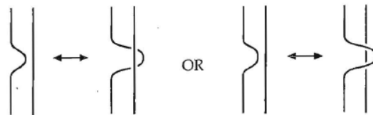
Figure 1.23 Type II Reidemeister move.
